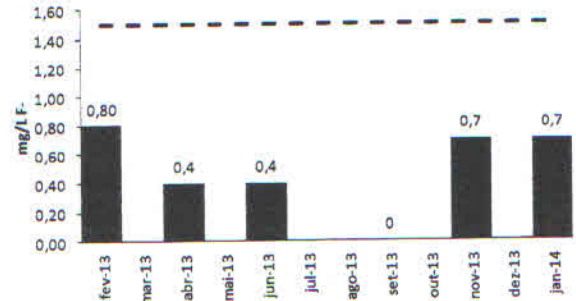
Figura 2 - Fluoreto (mg/L)
